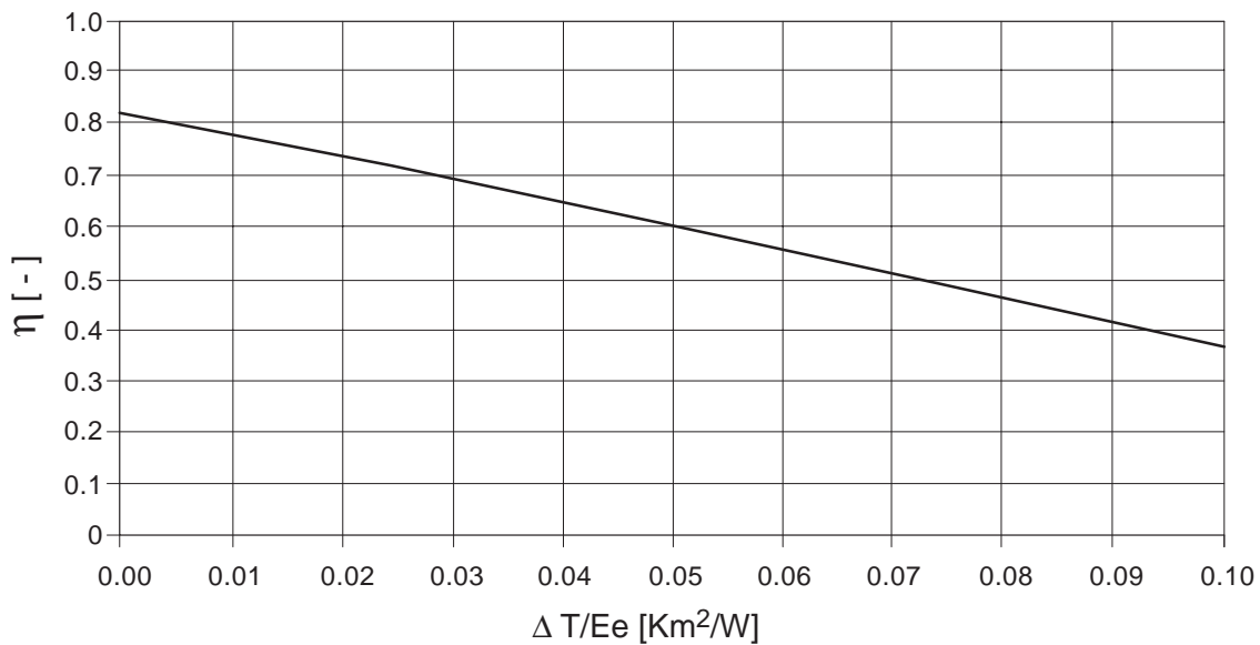
Efficiency characteristic curve [Ee = 800 W/m 2 ]
